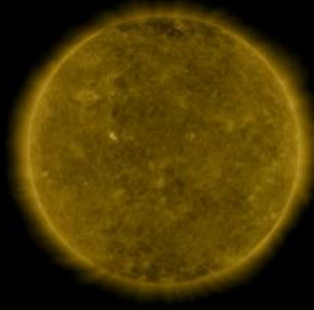
SOLAR MINIMUM
