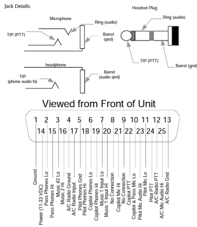
Figure 2 Connector Diagram (Unit has Male Pins)
