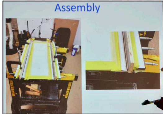
Side Panels
