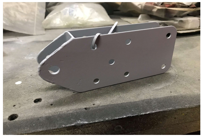
Right Wing Front Spar Attach Bracket - After
