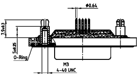
Shellsize 1-4
