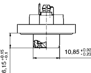
Shellsize 5
