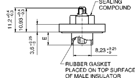
Shellsize 1-4
